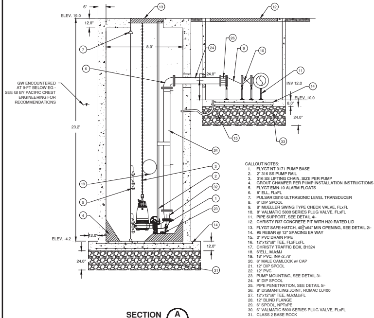
SECTION A
