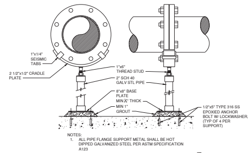
PIPE SUPPORT
