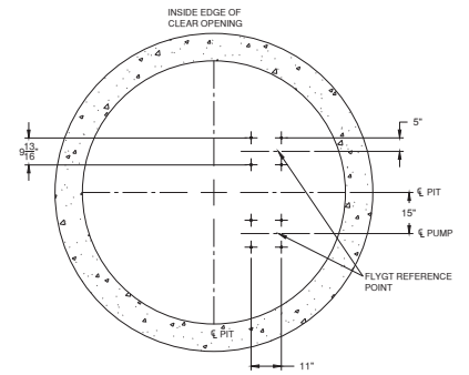
PUMP MOUNTING
