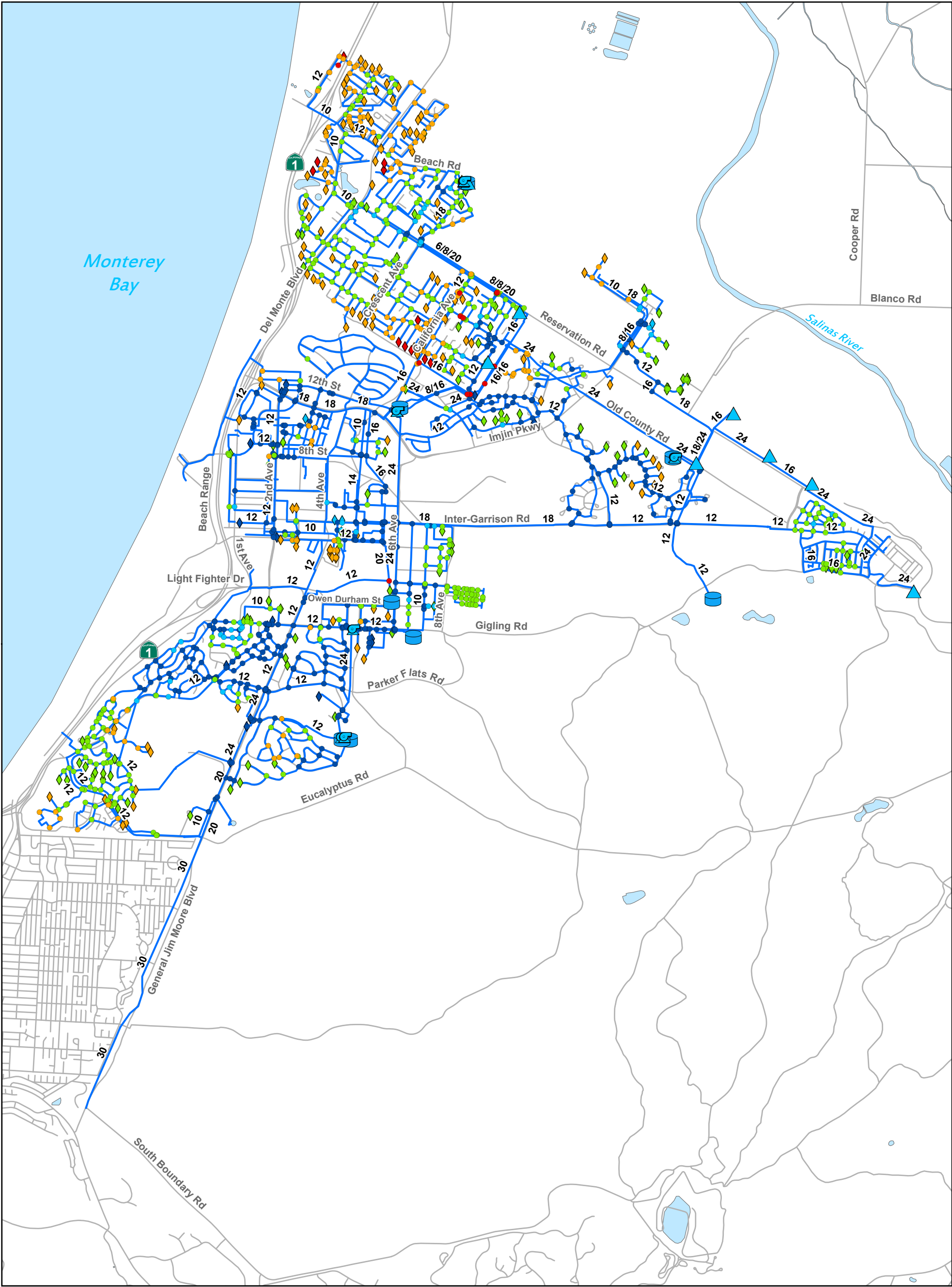
Figure 7.3 Available Fire Flow Water Master Plan Marina Coast Water District
